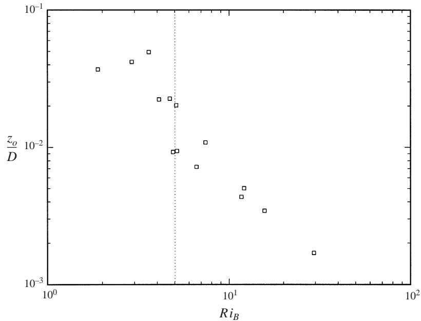
FIGURE 16. Interfacial roughness height normalized by the mixed-layer depth z_o/D as a function of Ri_B (two-layer case).
