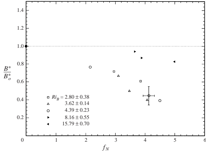
FIGURE 11. Buoyancy flux of linearly stratified experiments B^* normalized by B_o^* (two-layer case) versus the frequency ratio f_N = ND/\Delta U (open symbols, K-H regime; solid symbols, symmetric Hölmböe wave regime).
