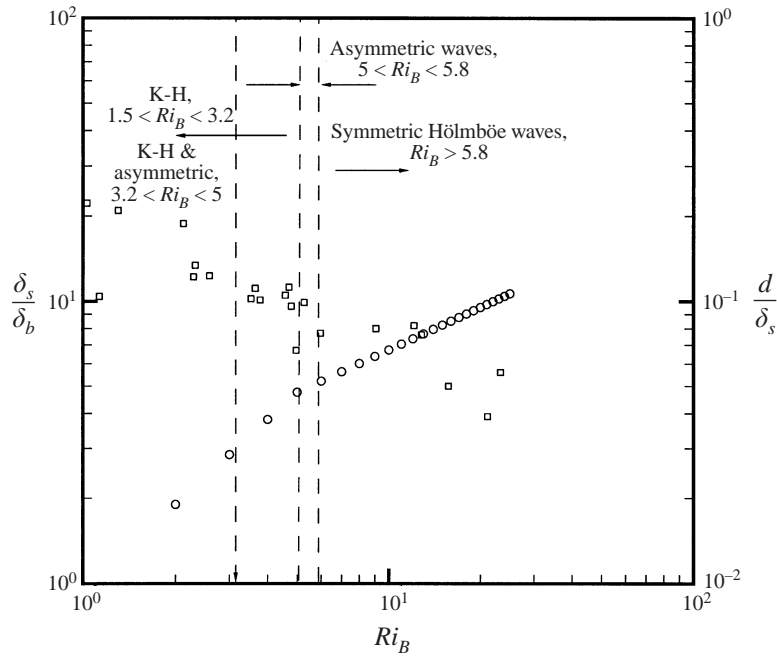
FIGURE 4. Ratio of velocity to density length scales \delta_s/\delta_b ( \circ ) and the normalized interfacial displacement d/\delta_s ( \square ) as a function of Ri_B . The regions of demarcation between K-H and symmetric Hölblöe instabilities are indicated.
