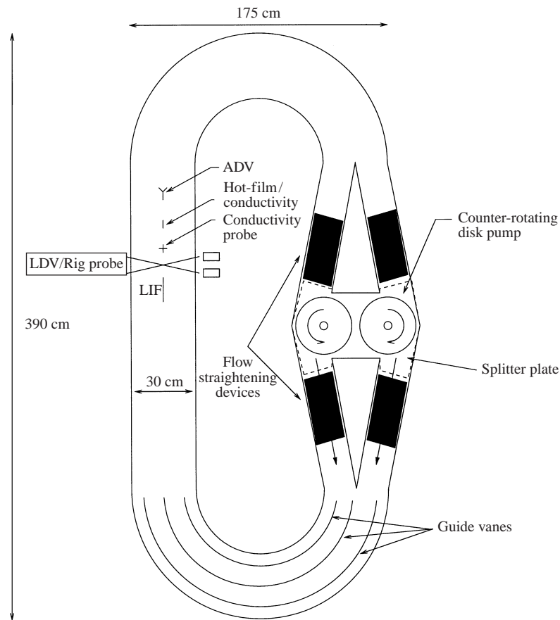
FIGURE 2. Schematic of closed-loop Odell-Kovaszny (recirculating) water facility.
